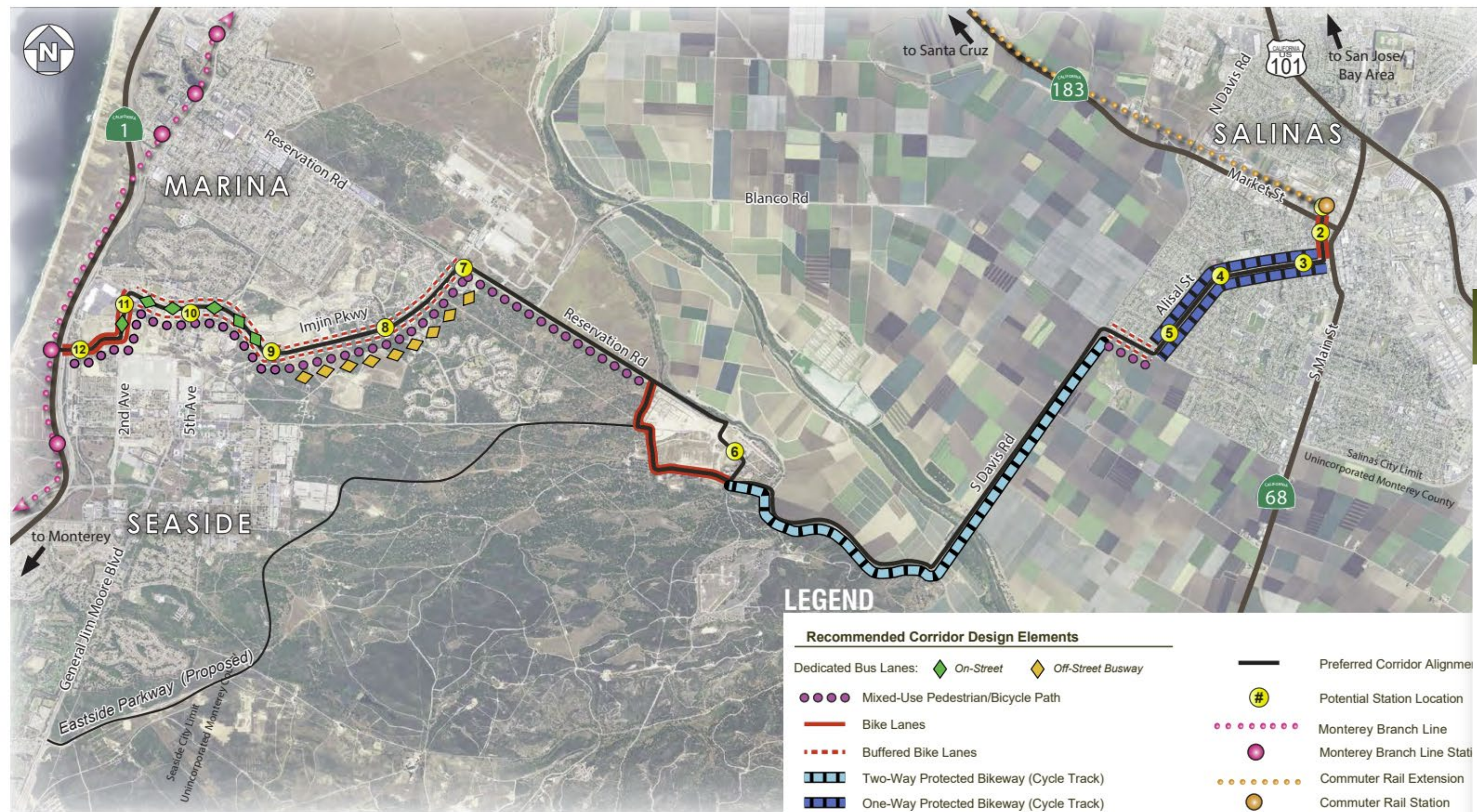
Figure 9-1: Preferred Alignment Configuration
