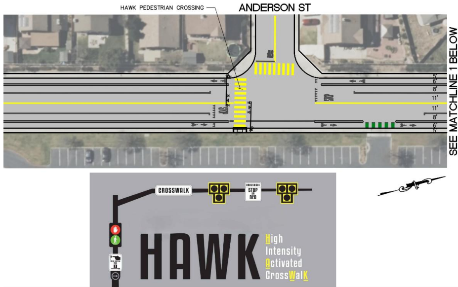
Figure 9 – ATP Proposed Safety Improvements Plans (Anderson at West)
