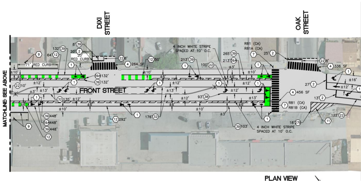
Figure 1- Front Street Striping Improvements
