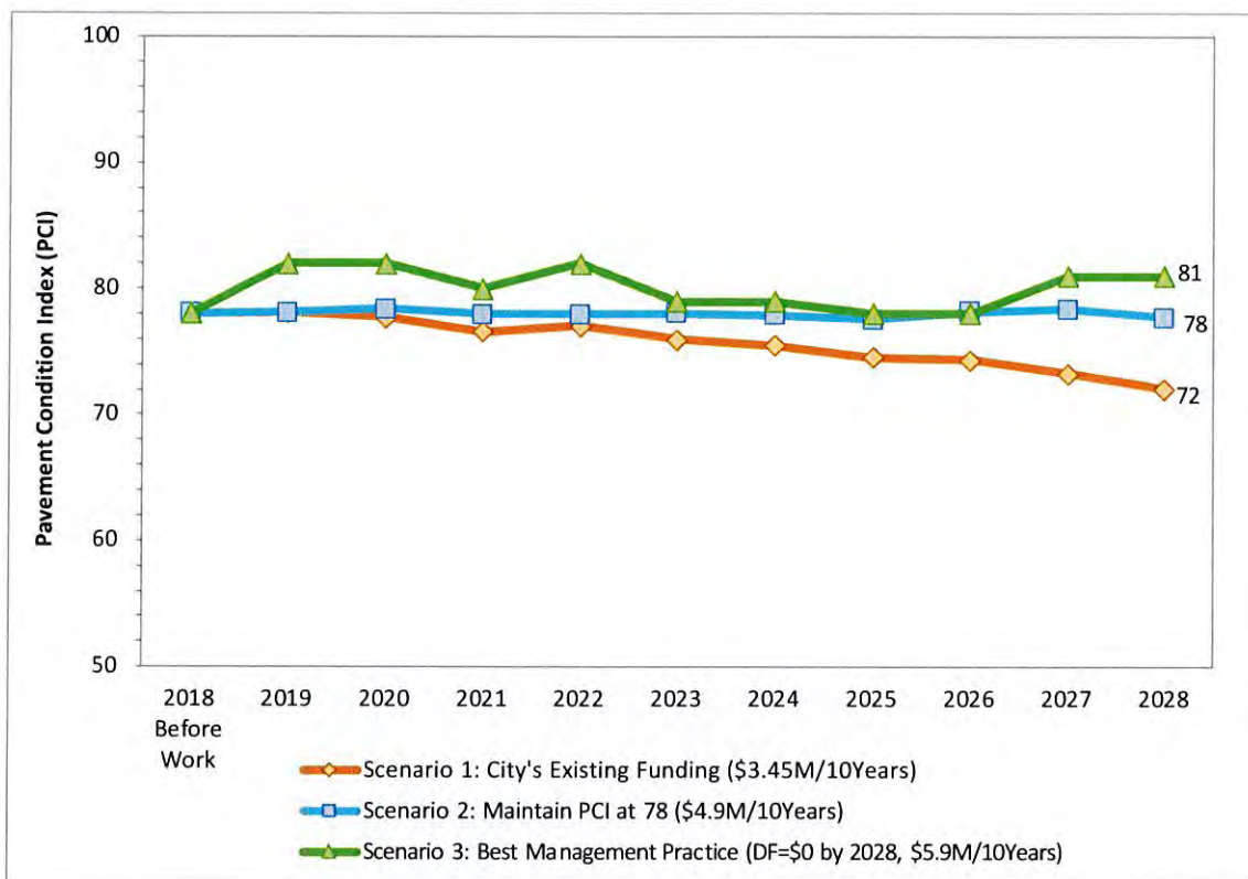
Figure 10: Annual Pavement Condition Index by Scenarios 1 to 3
