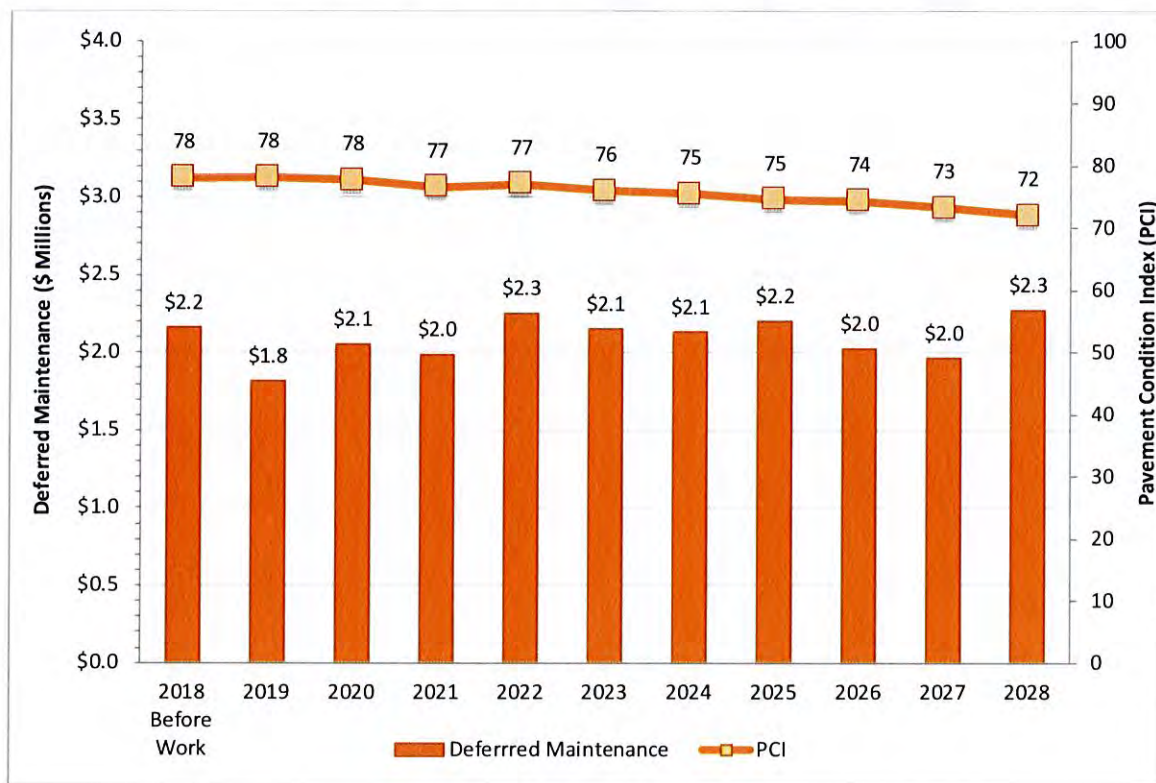
Figure 7: PCI vs Deferred Maintenance for Scenario 1
