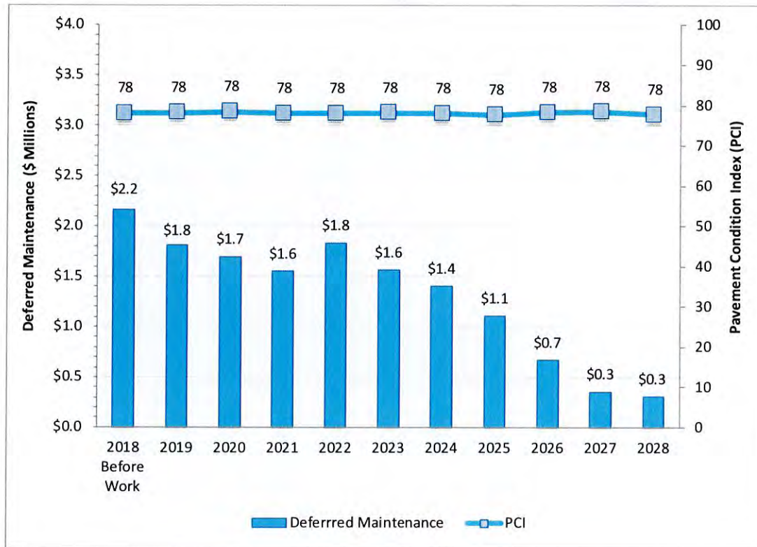
Figure 8: PCI vs Deferred Maintenance for Scenario 2
