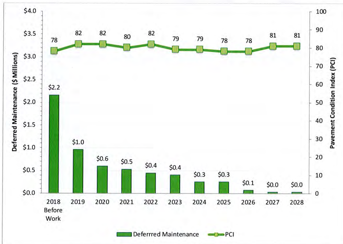
Figure 9: PCI vs Deferred Maintenance for Scenario 3
