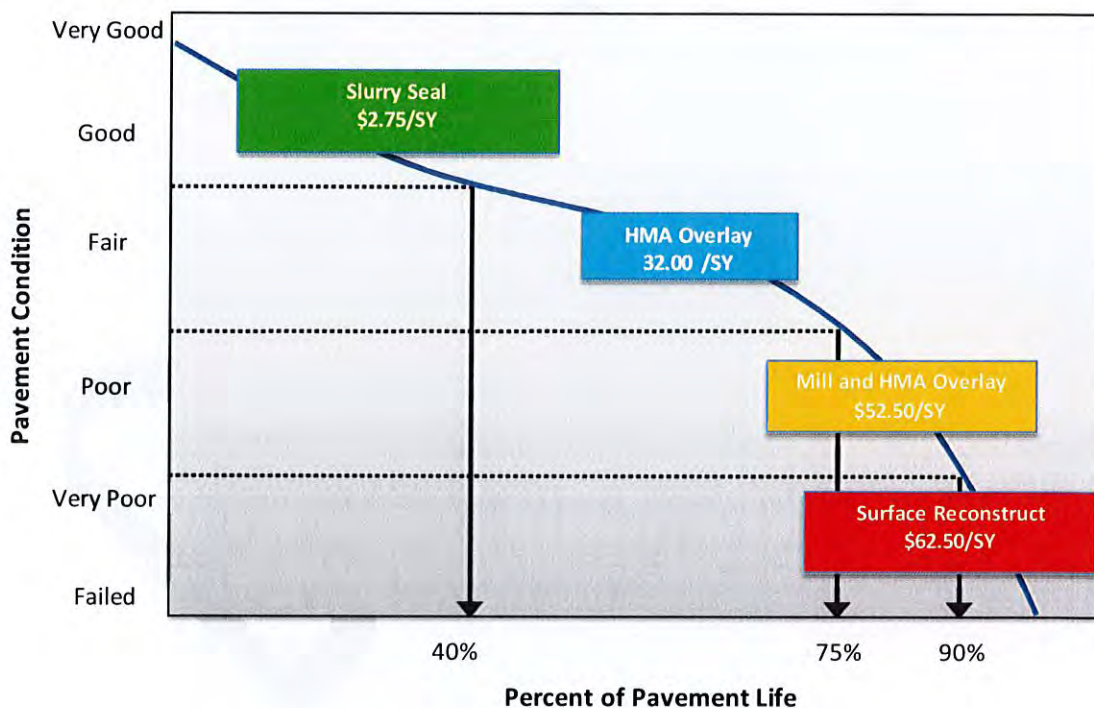
Figure 6: Costs of Maintaining Pavements over Time
